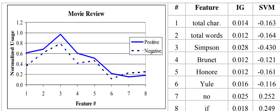
Fig. 4. Key Stylistic Features for Movie Review Data Set
