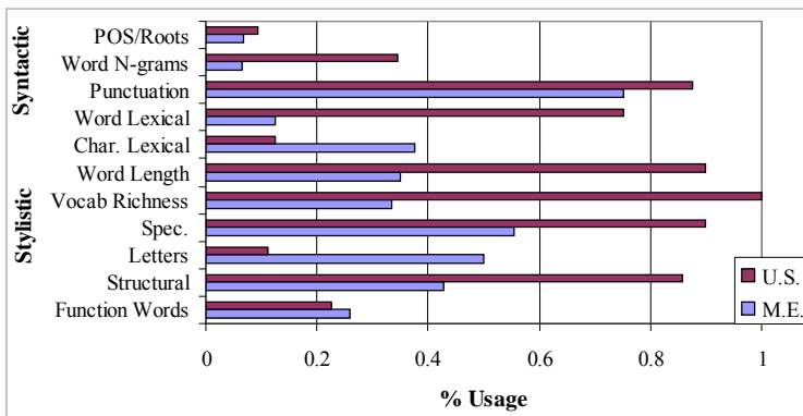
Fig. 7. Key feature usage percentage by category
