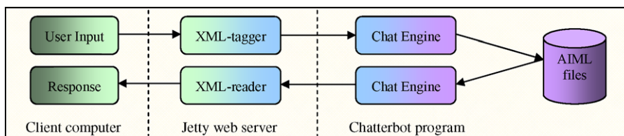
Fig. 1. Diagram of user input to chatterbot response.
