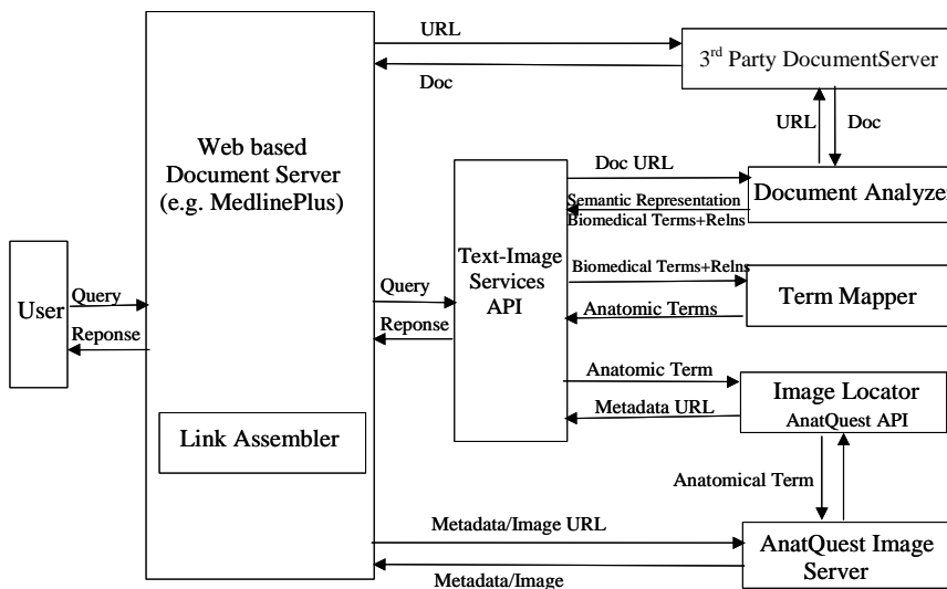
Figure 11-9. Architectural components for linking text and images.
